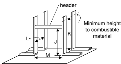
FRAMING - FRONT VIEW
